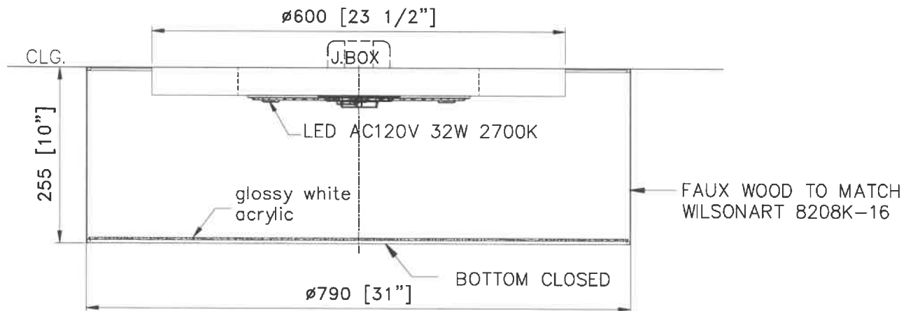
FRONT VIEW
