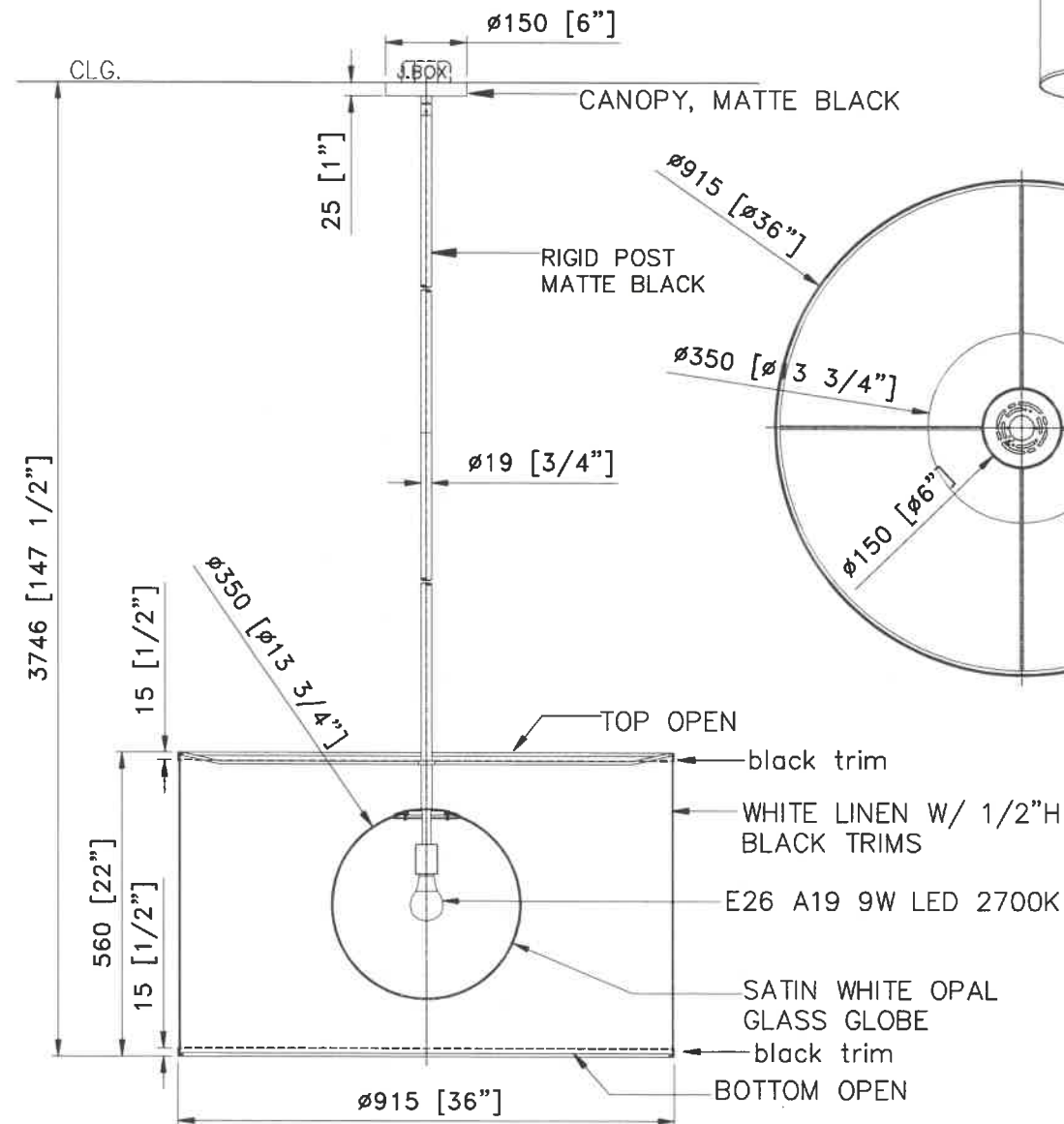
FRONT VIEW
